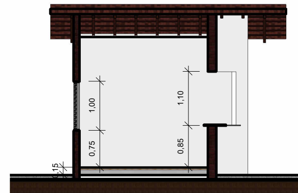
4 Section 1 ESCALA 1:75
