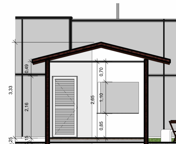
3 Section 0 ESCALA 1:75
